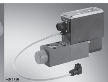
Type VT-DFPE-.-2X/... with integrated electronics
