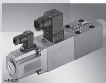
Type VT-DFP-.-2X/... with mating connector (separate order)
